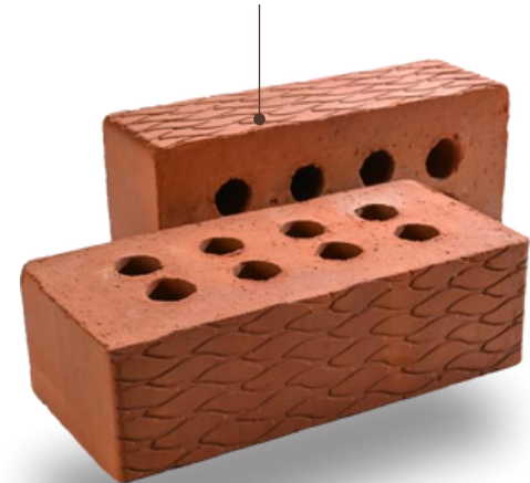
REB-75 LEAF BRICK Size 220 x 100 x 70 mm
