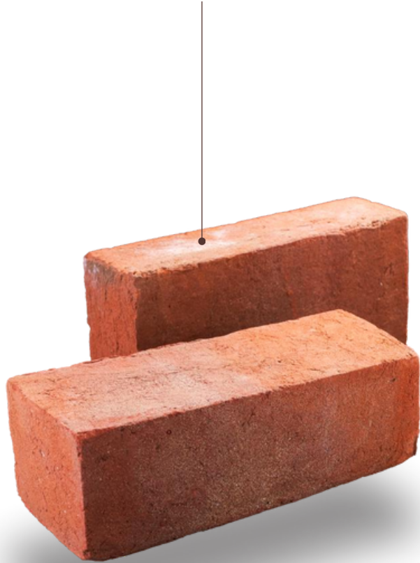
RHB-93 SOLID BRICK (No Frog) Size 215 x 100 x 65mm
