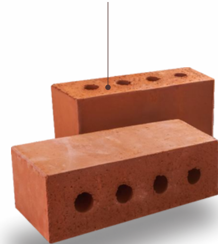
REB-92 (B) Rat Trap Facing Brick Size 220 x 100 x 70 mm
