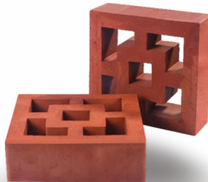
REJ-725 Smart Square Size 210 x 210 x 70mm
