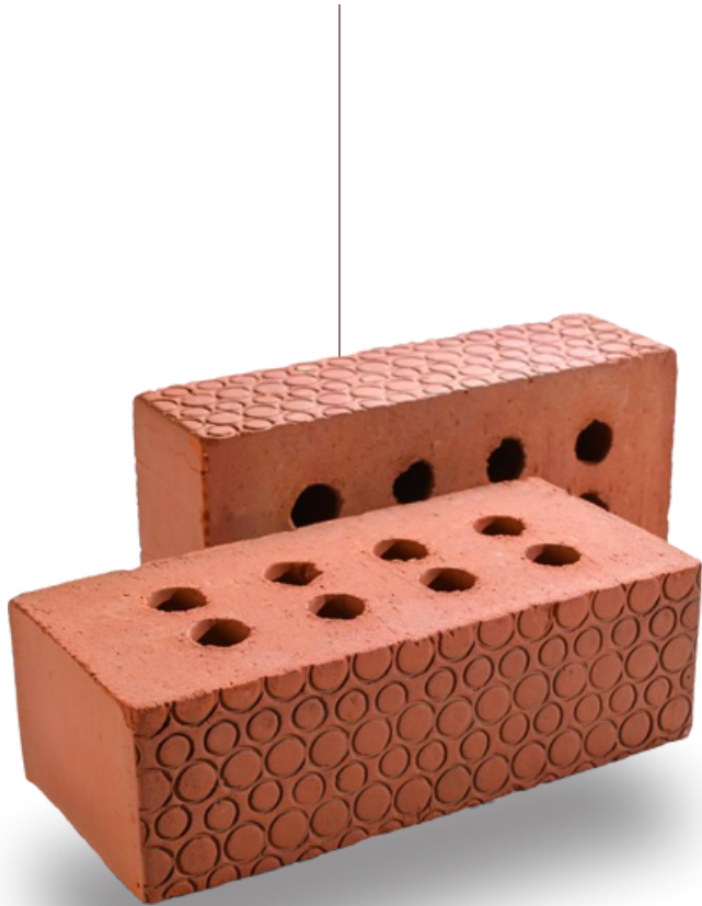
REB-83 BUBBL E BRICK Size 220 x 100 x 70 mm
